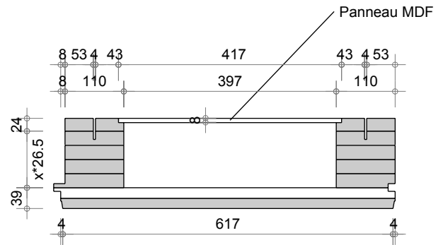
HBV Q2 Joint V de 7,9mm
