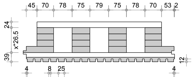
Dalle D Q4 coupe de long.
