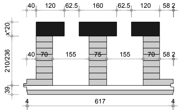
Dalle R Q3 BV Joint V de 7,9mm
