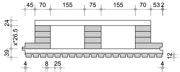
Dalle D Q3 coupe long.
